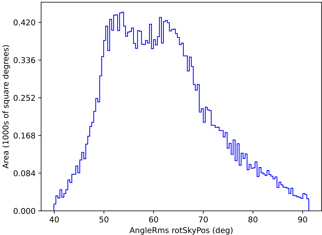
too_ignore_10_1v3.4_10yrs All sky i band: AngleRms rotSkyPos
