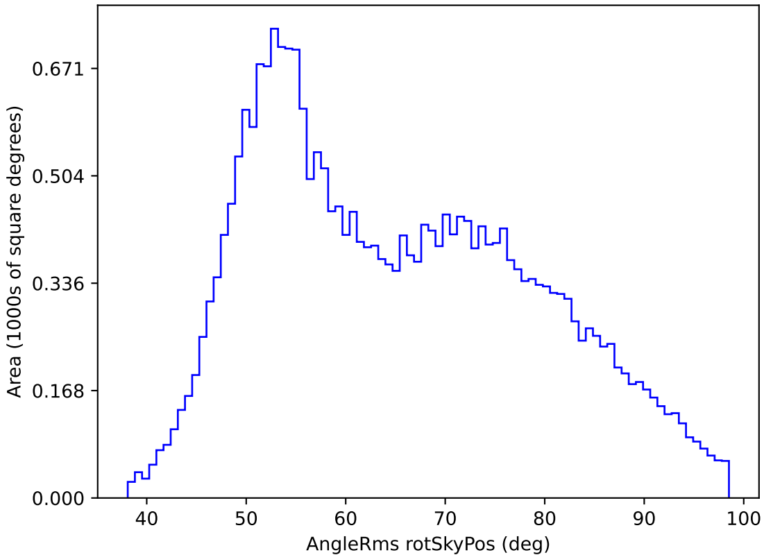
too_ignore_10_1v3.4_10yrs All sky g band: AngleRms rotSkyPos
