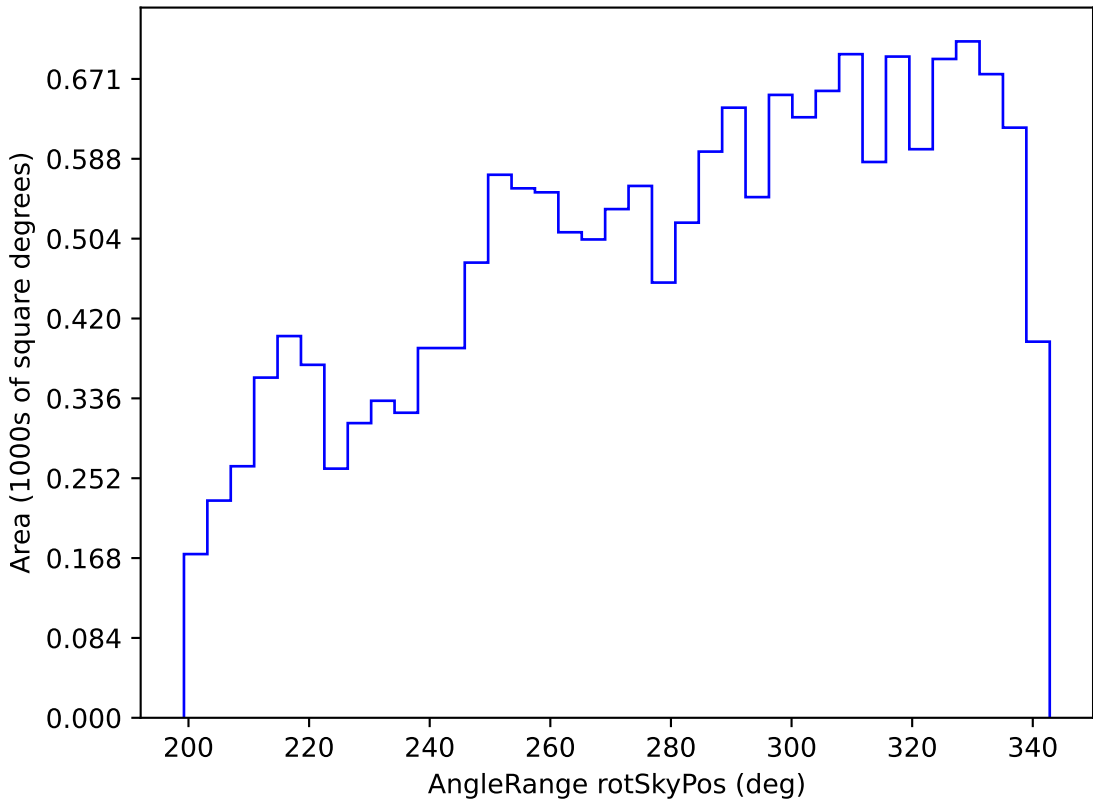
too_ignore_10_1v3.4_10yrs WFD z band: AngleRange rotSkyPos
