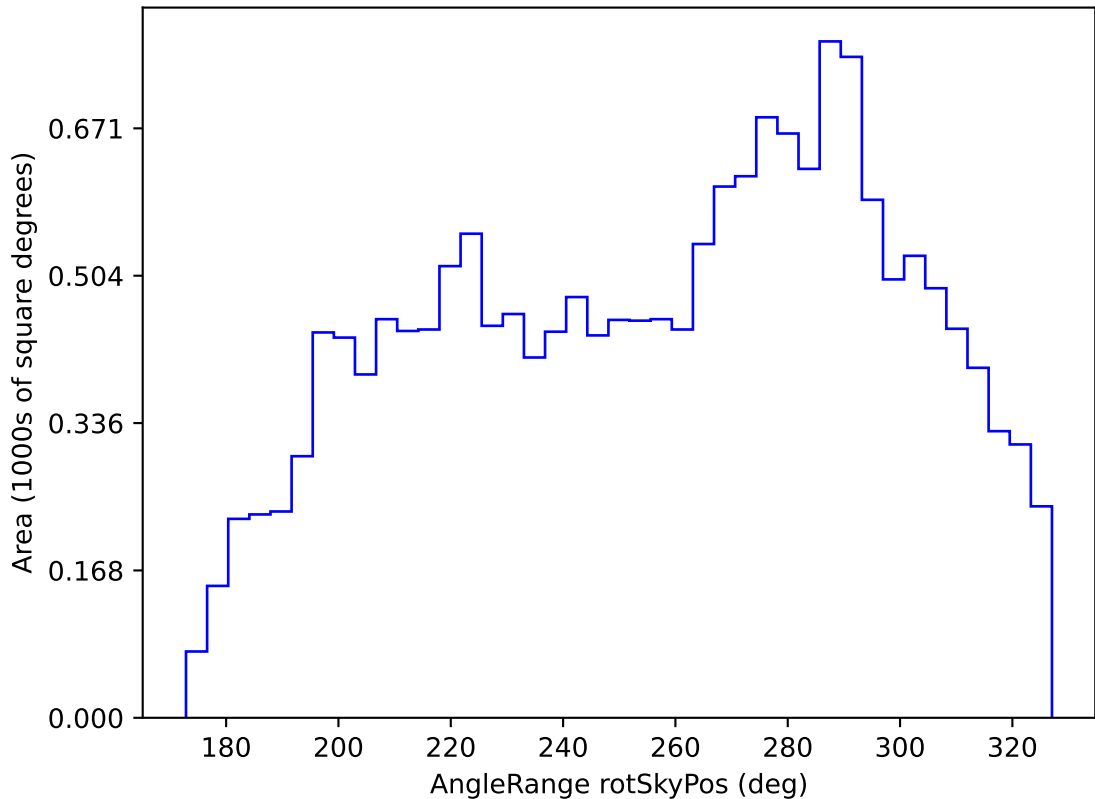
too_ignore_10_1v3.4_10yrs WFD u band: AngleRange rotSkyPos
