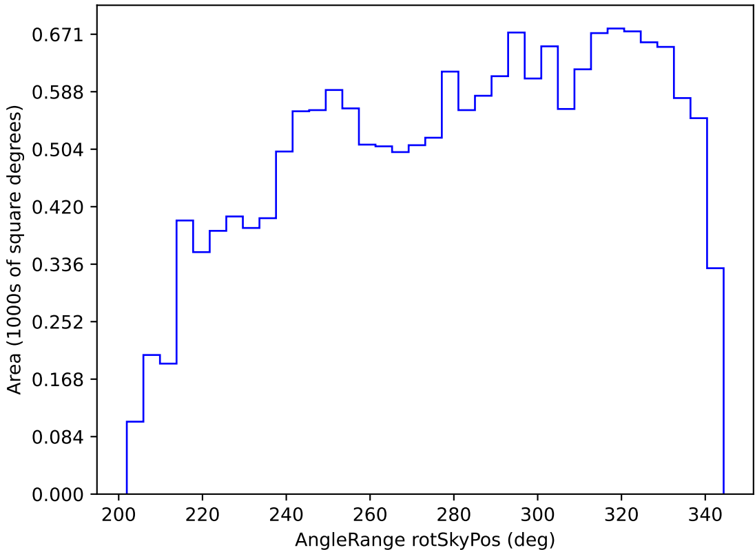
too_ignore_10_1v3.4_10yrs WFD r band: AngleRange rotSkyPos
