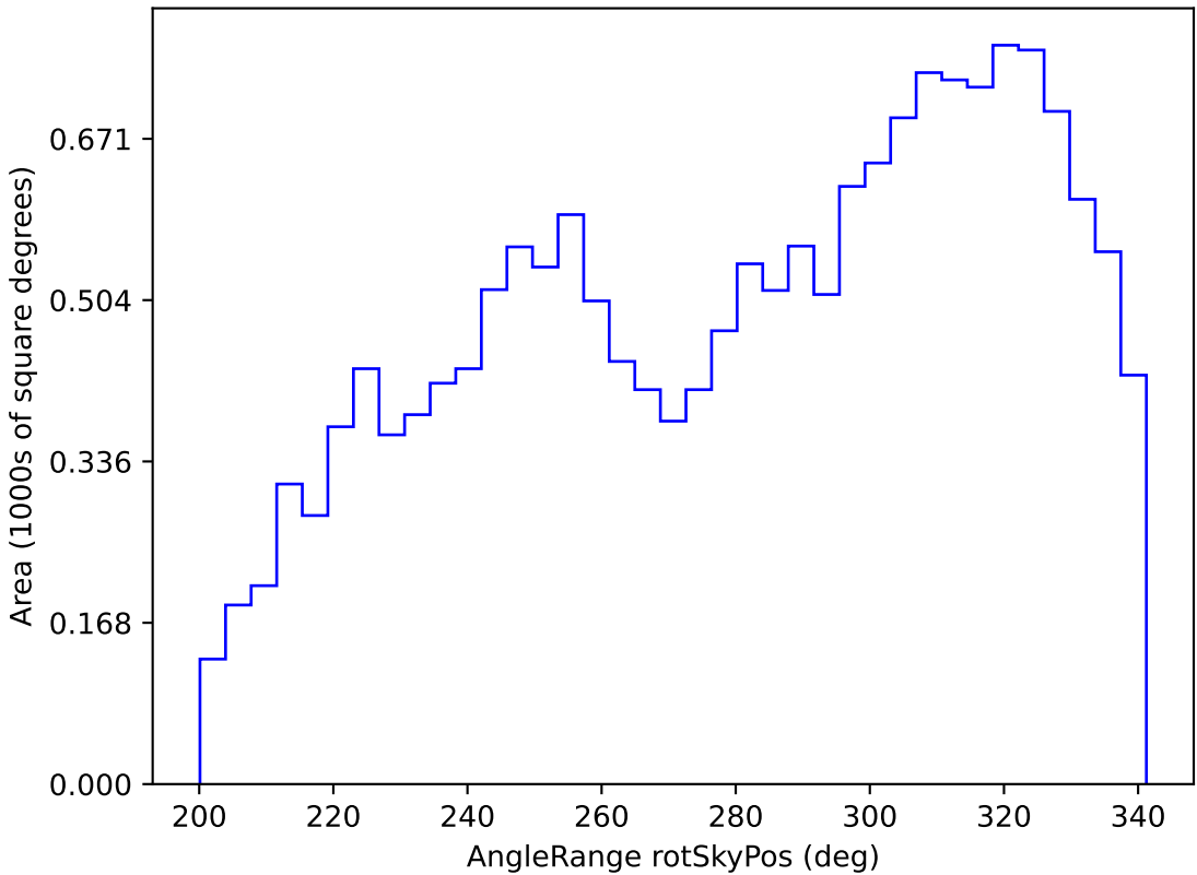
too_ignore_10_1v3.4_10yrs WFD i band: AngleRange rotSkyPos
