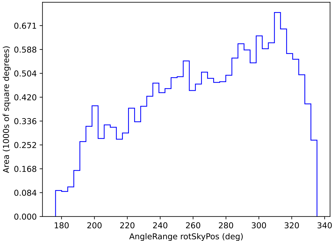
too_ignore_10_1v3.4_10yrs WFD g band: AngleRange rotSkyPos
