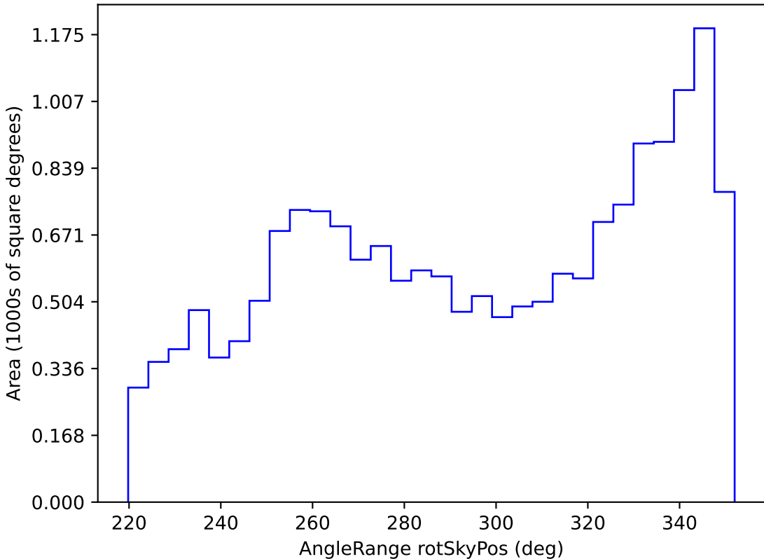
too_ignore_10_1v3.4_10yrs WFD all bands: AngleRange rotSkyPos
