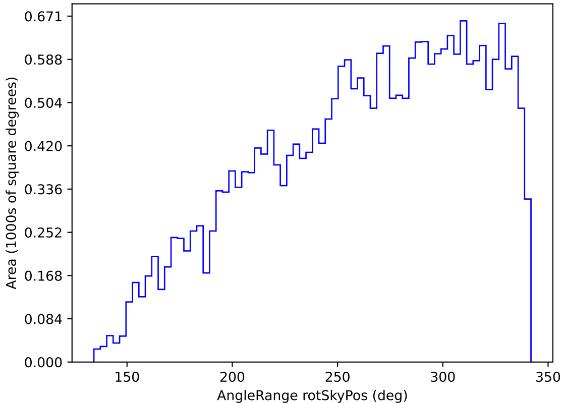
too_ignore_10_1v3.4_10yrs All sky z band: AngleRange rotSkyPos
