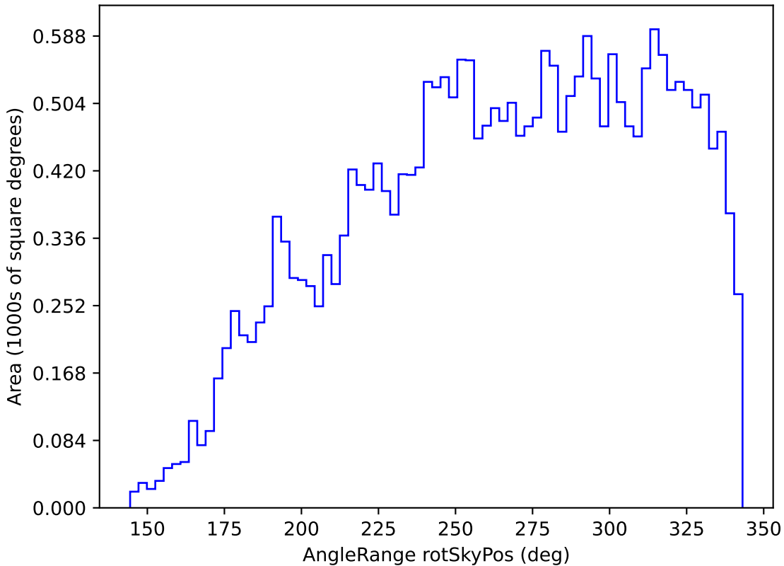
too_ignore_10_1v3.4_10yrs All sky r band: AngleRange rotSkyPos
