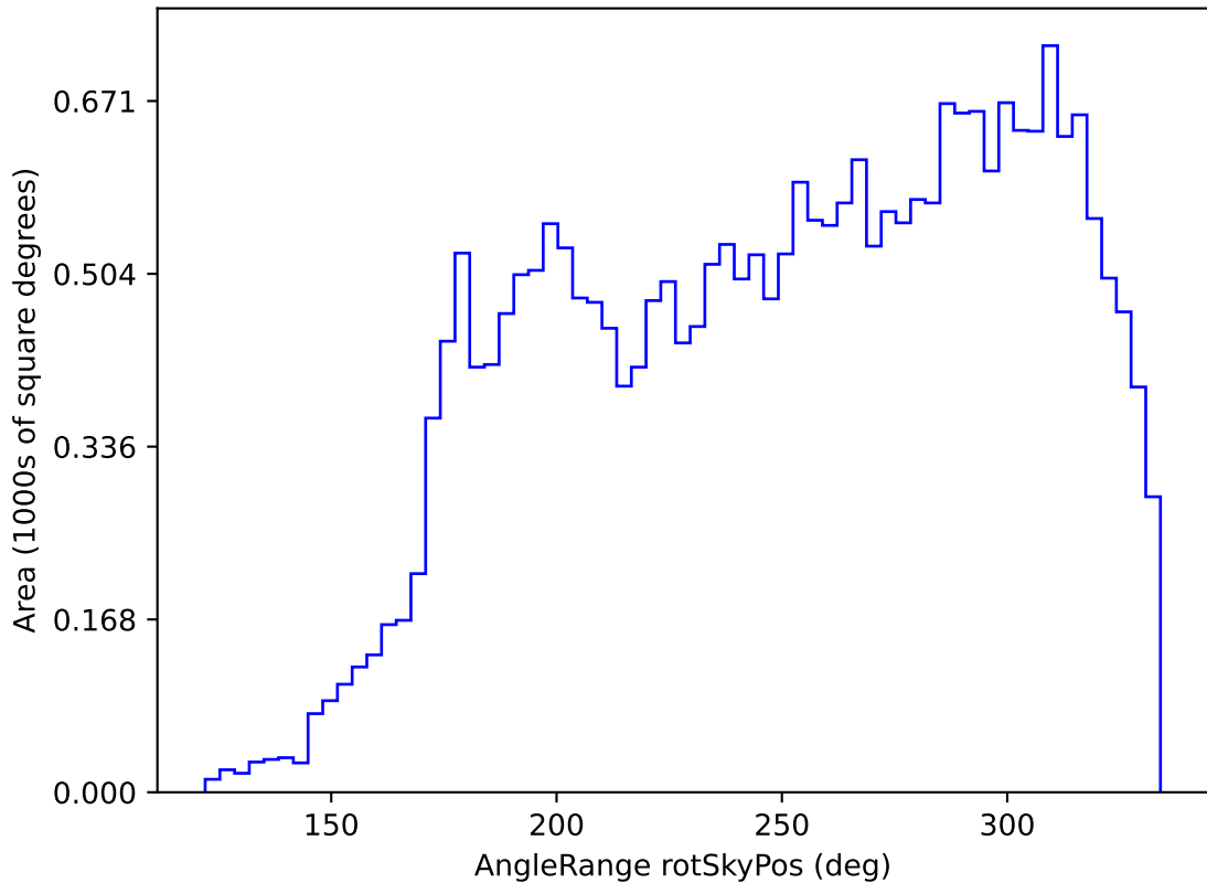
too_ignore_10_1v3.4_10yrs All sky g band: AngleRange rotSkyPos
