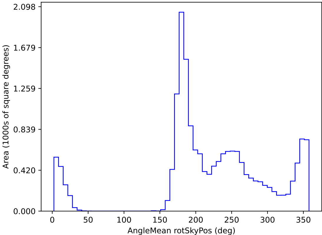
too_ignore_10_1v3.4_10yrs WFD z band: AngleMean rotSkyPos
