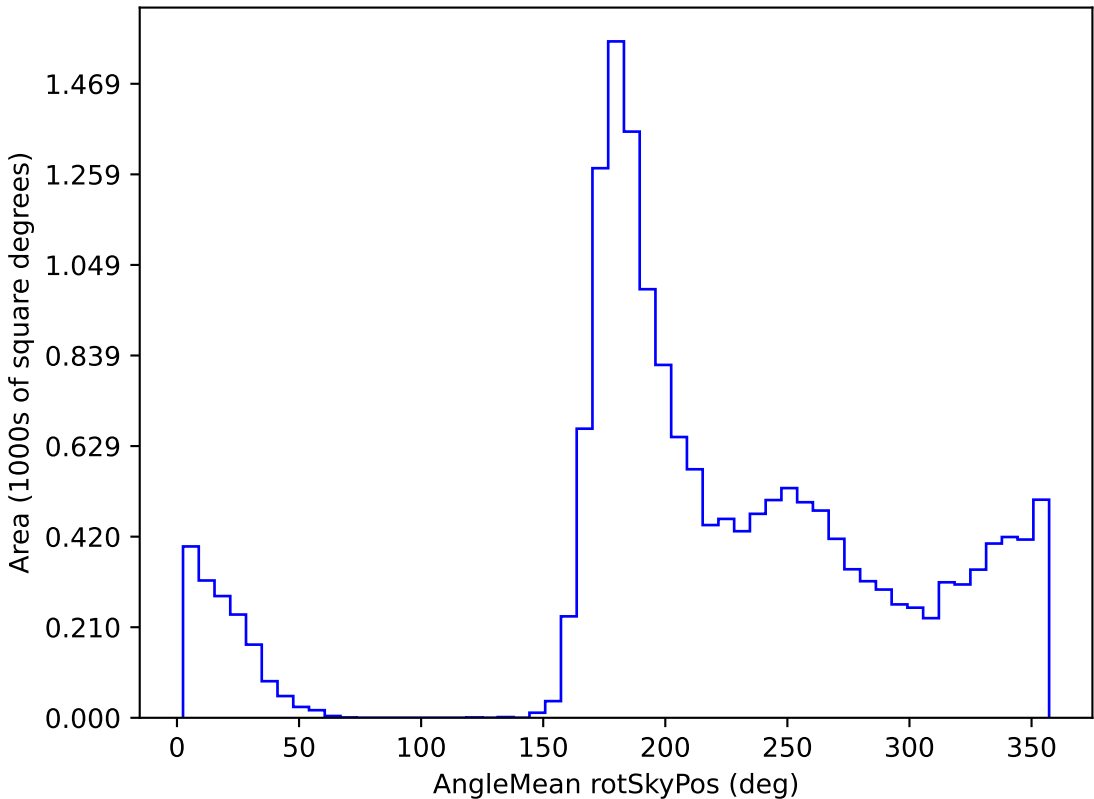
too_ignore_10_1v3.4_10yrs WFD u band: AngleMean rotSkyPos
