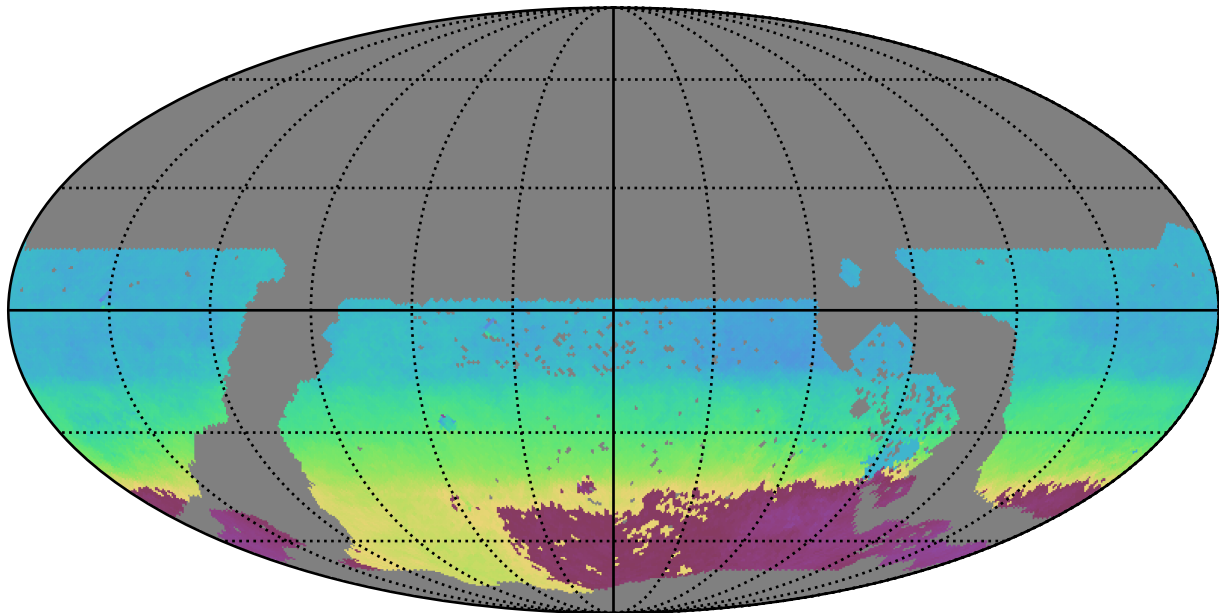
too_ignore_10_1v3.4_10yrs WFD r band: AngleMean rotSkyPos
