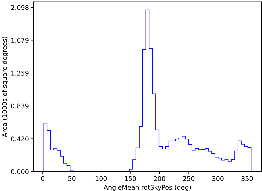
too_ignore_10_1v3.4_10yrs WFD r band: AngleMean rotSkyPos
