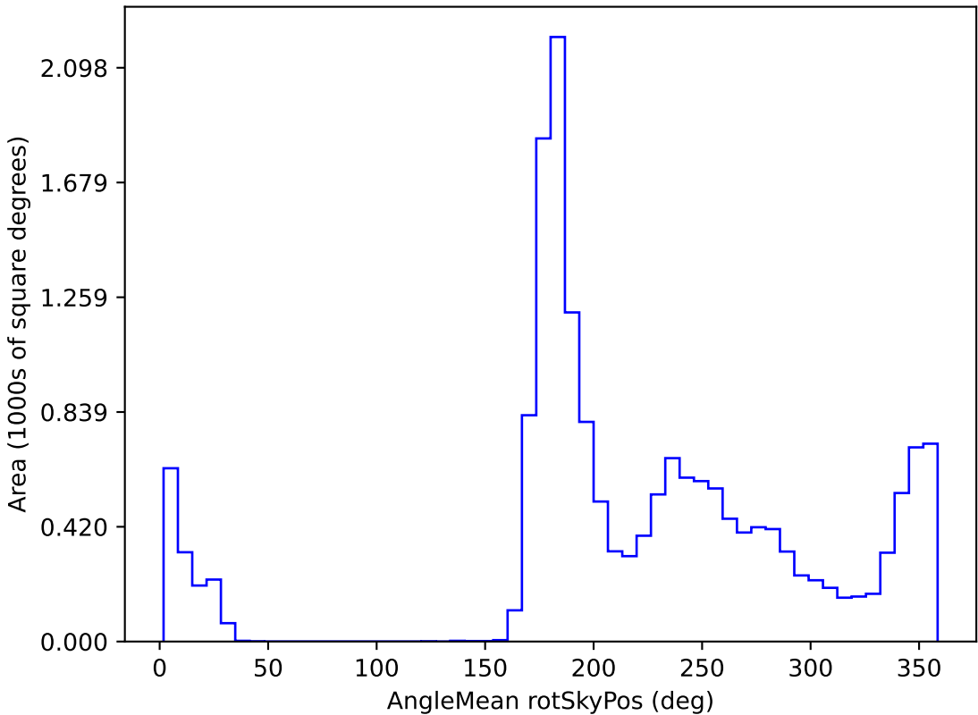
too_ignore_10_1v3.4_10yrs WFD i band: AngleMean rotSkyPos
