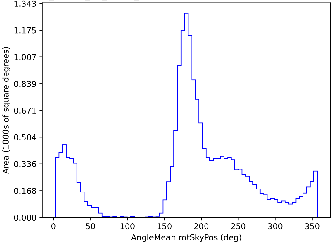
too_ignore_10_1v3.4_10yrs WFD g band: AngleMean rotSkyPos
