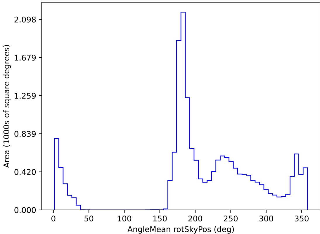
too_ignore_10_1v3.4_10yrs WFD all bands: AngleMean rotSkyPos
