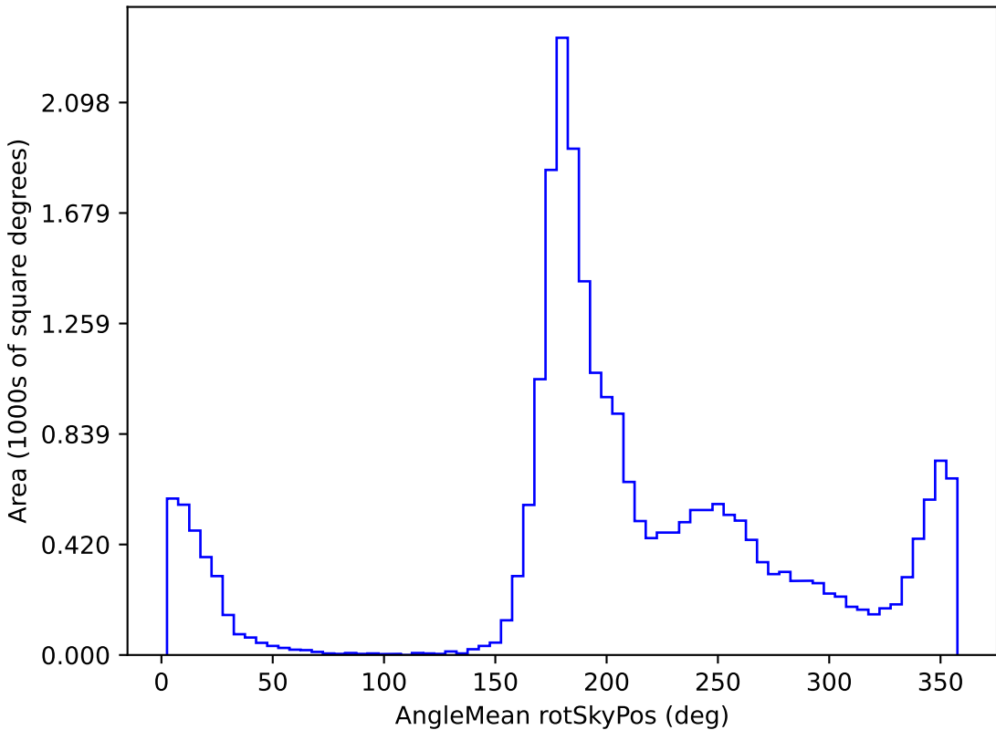
too_ignore_10_1v3.4_10yrs All sky z band: AngleMean rotSkyPos
