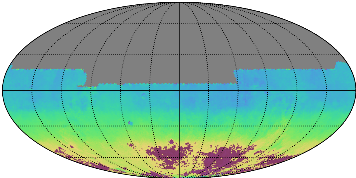
too_ignore_10_1v3.4_10yrs All sky y band: AngleMean rotSkyPos
