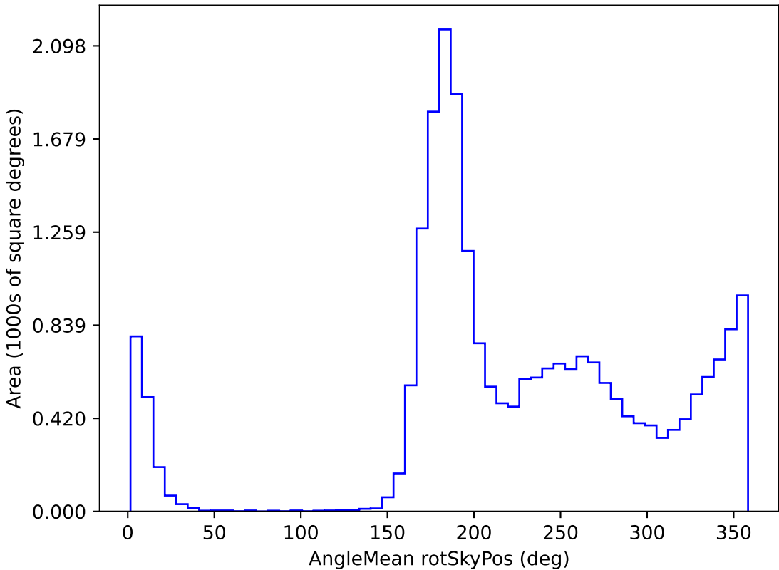
too_ignore_10_1v3.4_10yrs All sky y band: AngleMean rotSkyPos
