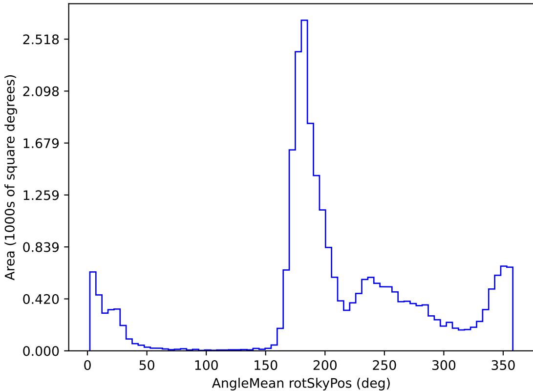
too_ignore_10_1v3.4_10yrs All sky i band: AngleMean rotSkyPos
