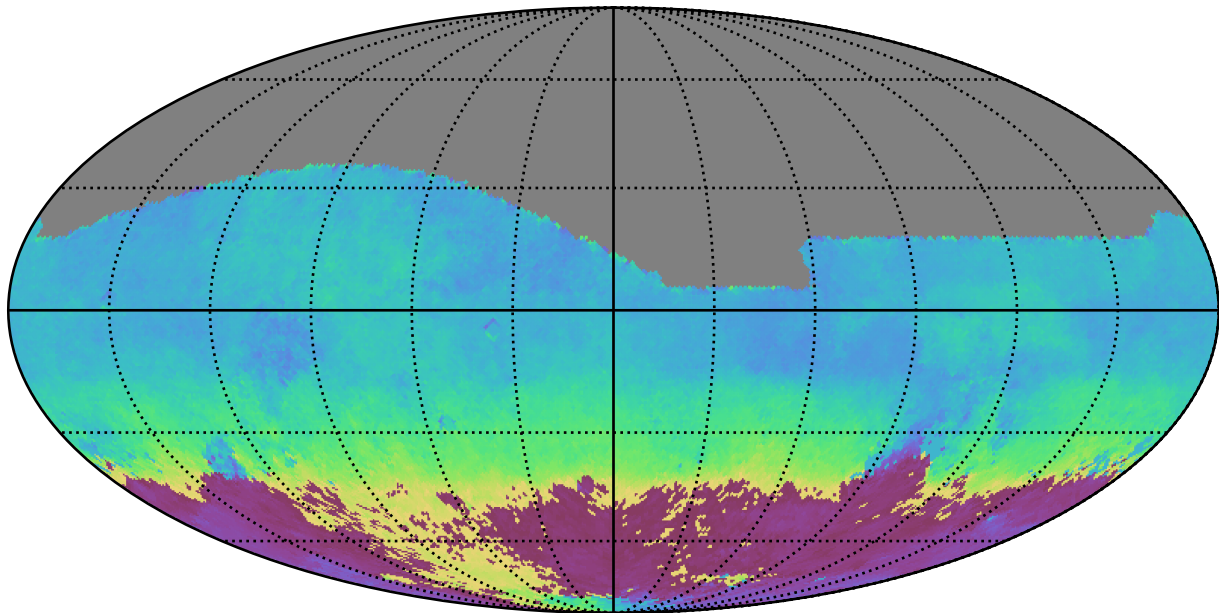
too_ignore_10_1v3.4_10yrs All sky g band: AngleMean rotSkyPos
