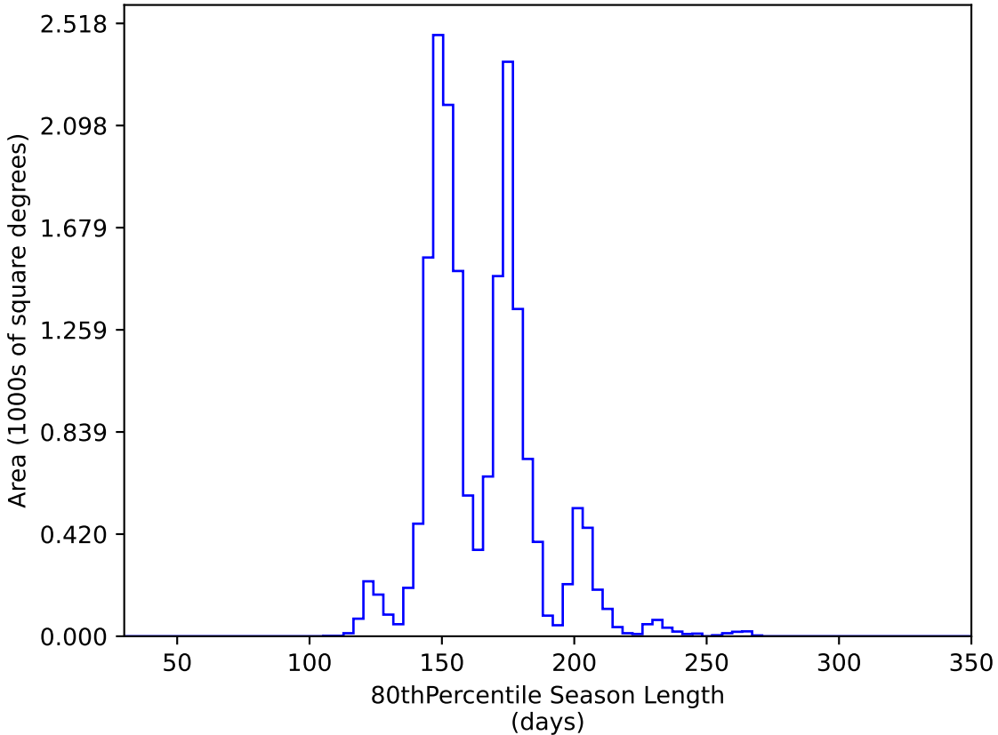
too_ignore_10_1v3.4_10yrs WFD y band: 80thPercentile Season Length
