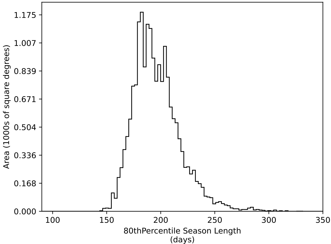
too_ignore_10_1v3.4_10yrs WFD all bands: 80thPercentile Season Length
