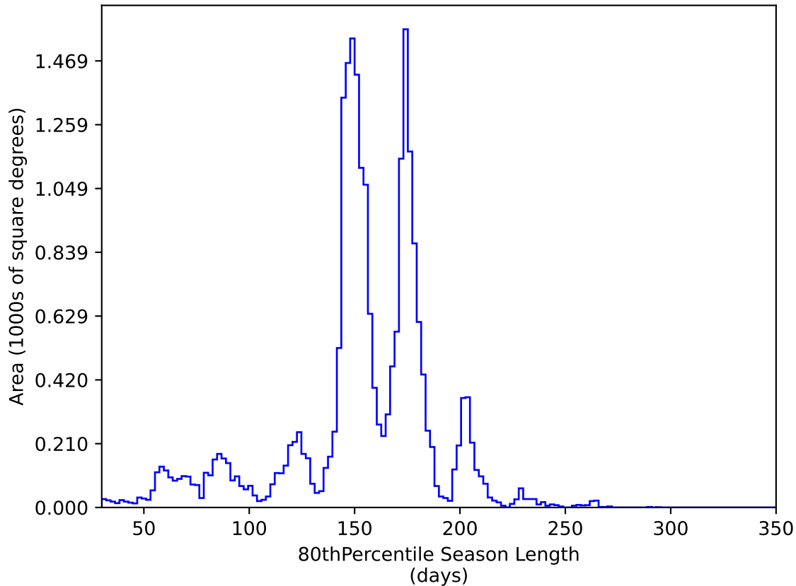
too_ignore_10_1v3.4_10yrs All sky y band: 80thPercentile Season Length
