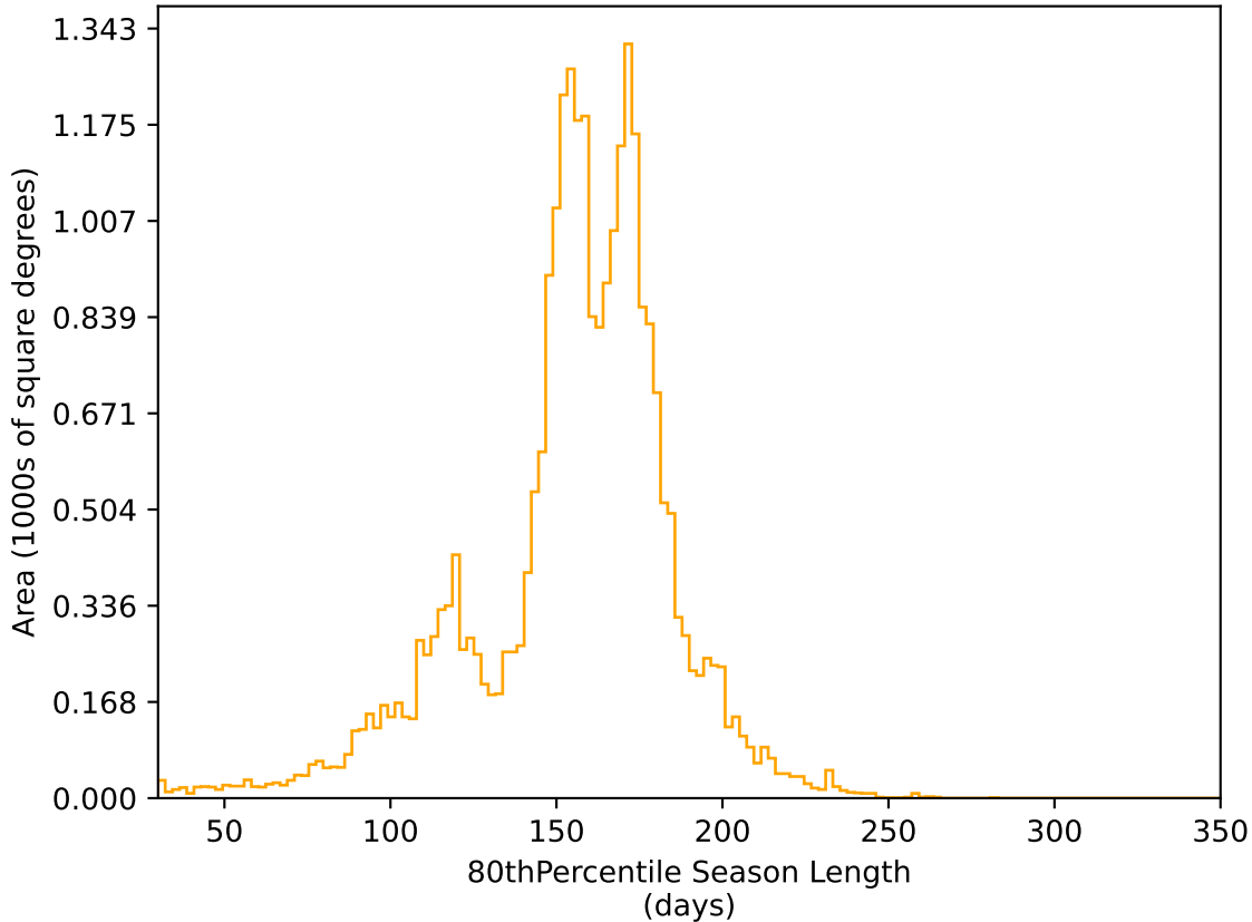
too_ignore_10_1v3.4_10yrs All sky r band: 80thPercentile Season Length
