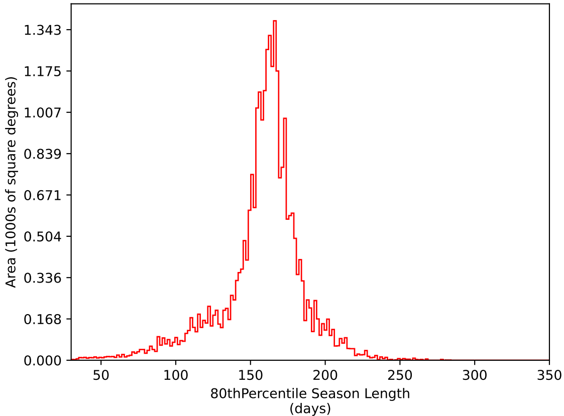
too_ignore_10_1v3.4_10yrs All sky i band: 80thPercentile Season Length
