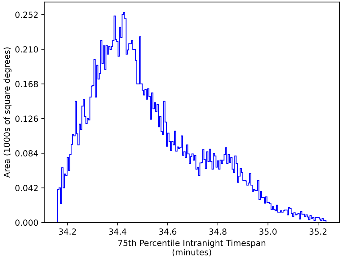
too_ignore_10_1v3.4_10yrs WFD zy bands: 75th Percentile Intranight Timespan
