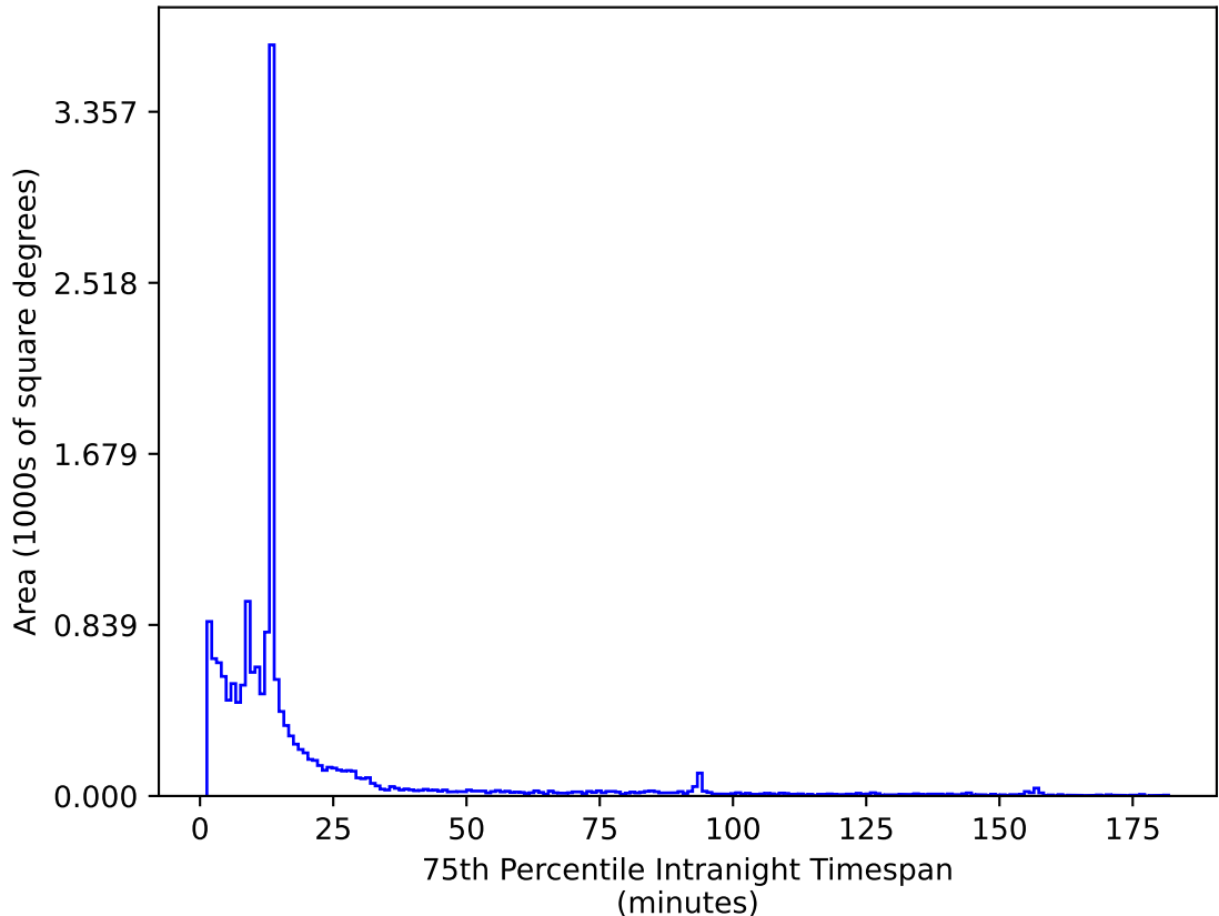
too_ignore_10_1v3.4_10yrs WFD z band: 75th Percentile Intranight Timespan
