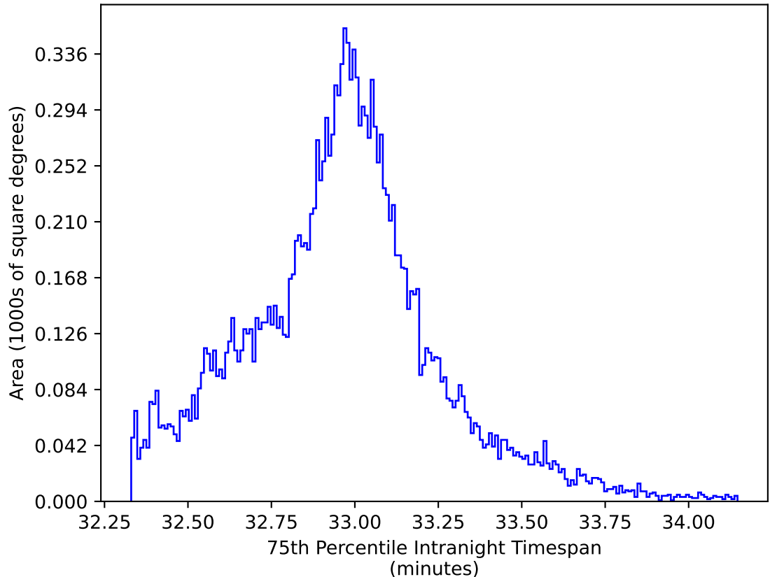
too_ignore_10_1v3.4_10yrs WFD y band: 75th Percentile Intranight Timespan
