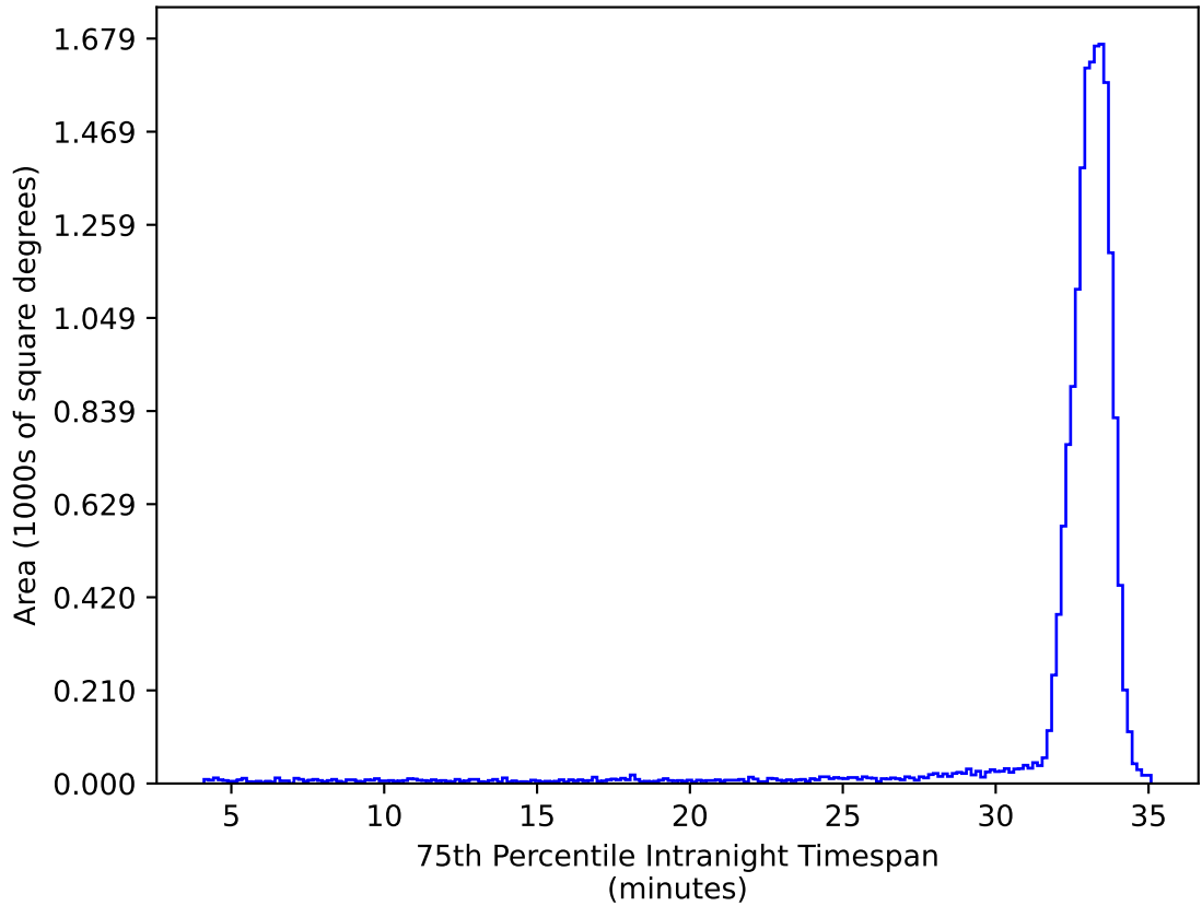
too_ignore_10_1v3.4_10yrs WFD ug bands: 75th Percentile Intranight Timespan
