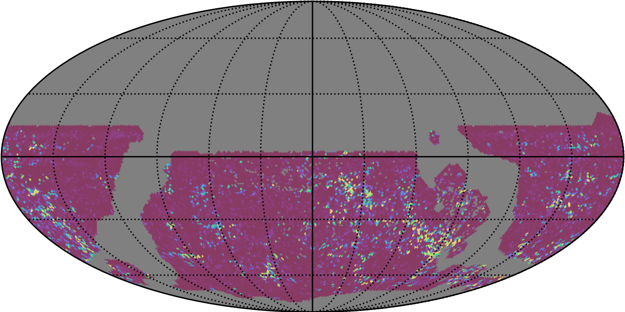
too_ignore_10_1v3.4_10yrs WFD u band: 75th Percentile Intranight Timespan
