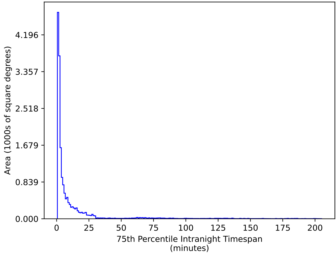
too_ignore_10_1v3.4_10yrs WFD u band: 75th Percentile Intranight Timespan
