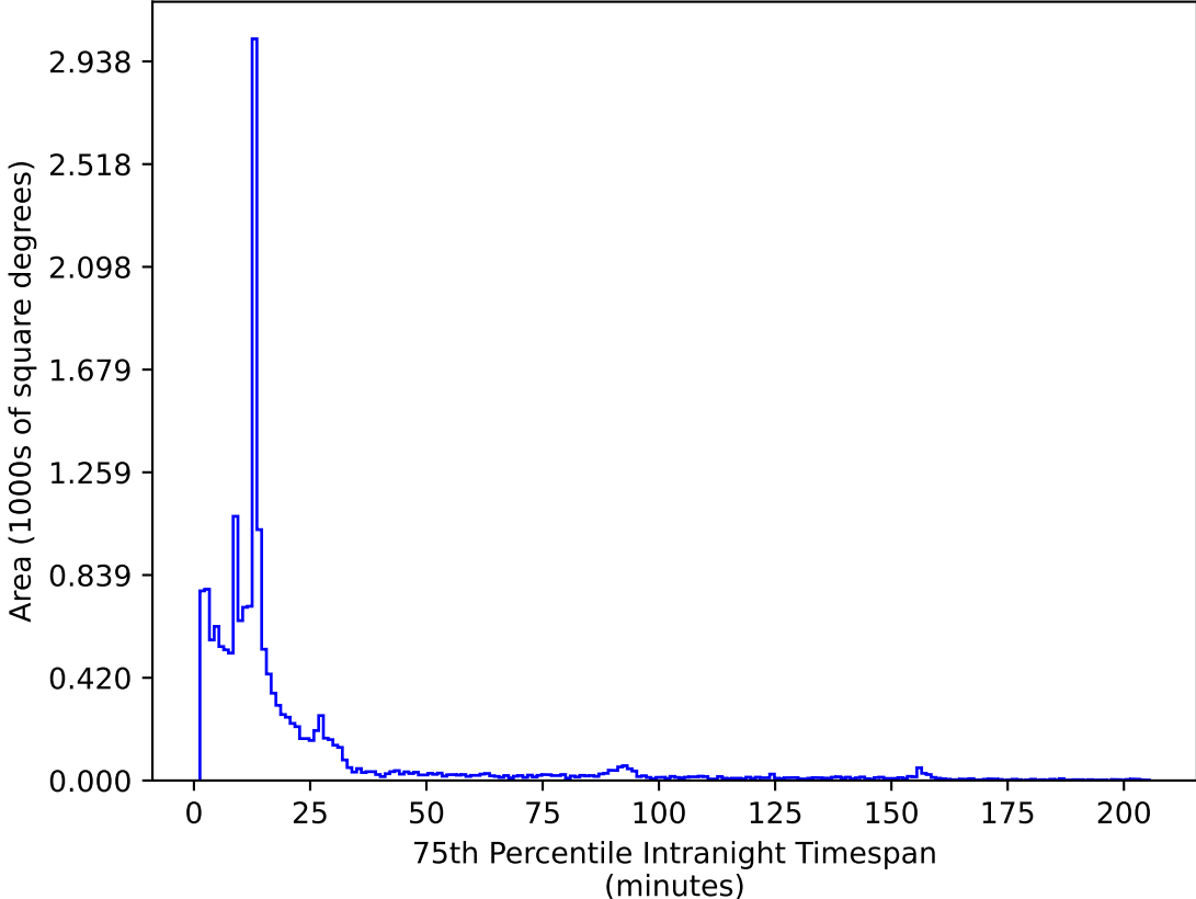
too_ignore_10_1v3.4_10yrs WFD i band: 75th Percentile Intranight Timespan
