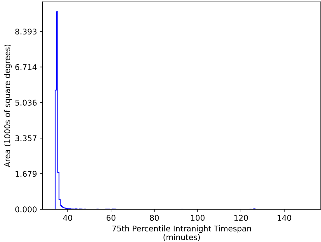
too_ignore_10_1v3.4_10yrs WFD gr bands: 75th Percentile Intranight Timespan
