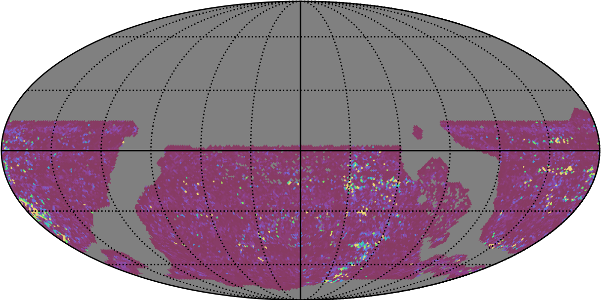
too_ignore_10_1v3.4_10yrs WFD g band: 75th Percentile Intranight Timespan
