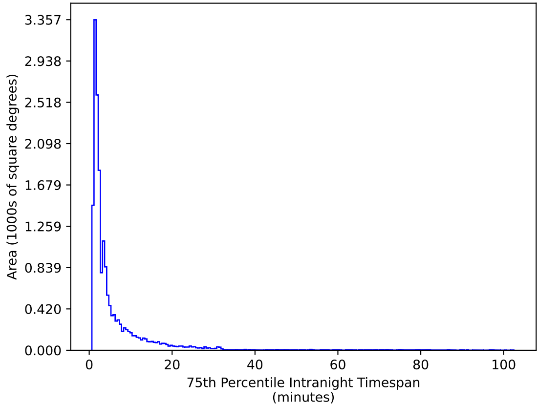
too_ignore_10_1v3.4_10yrs WFD g band: 75th Percentile Intranight Timespan
