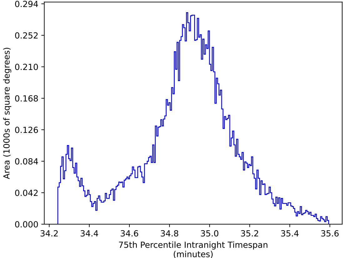
too_ignore_10_1v3.4_10yrs WFD all bands: 75th Percentile Intranight Timespan
