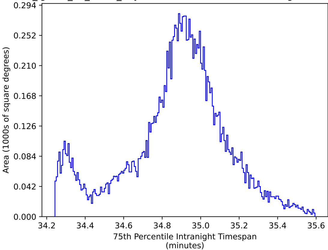
too_ignore_10_1v3.4_10yrs WFD: 75th Percentile Intranight Timespan
