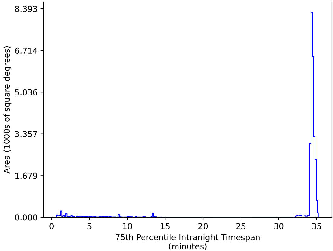
too_ignore_10_1v3.4_10yrs All sky zy bands: 75th Percentile Intranight Timespan
