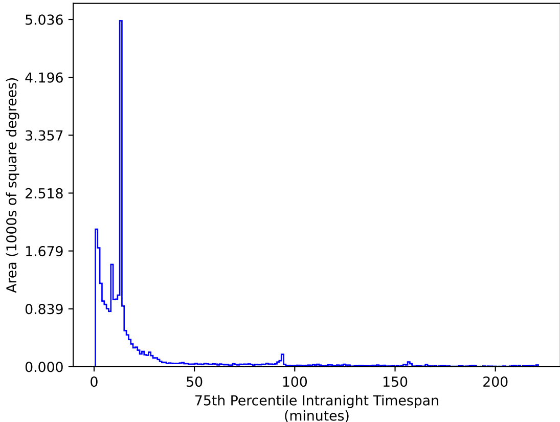
too_ignore_10_1v3.4_10yrs All sky z band: 75th Percentile Intranight Timespan
