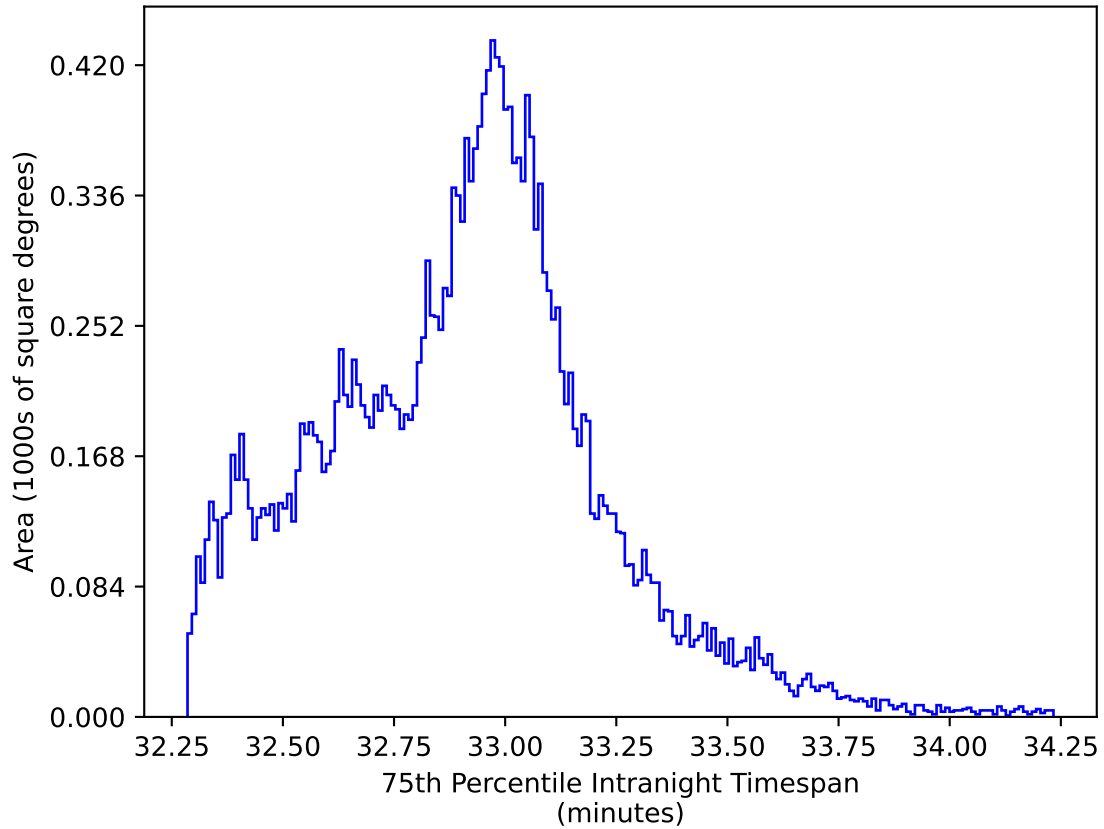
too_ignore_10_1v3.4_10yrs All sky y band: 75th Percentile Intranight Timespan
