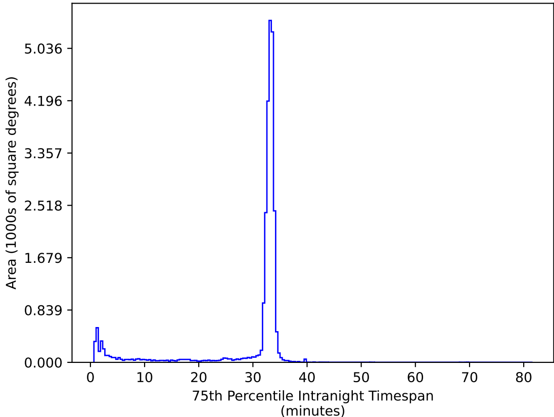
too_ignore_10_1v3.4_10yrs All sky ug bands: 75th Percentile Intranight Timespan
