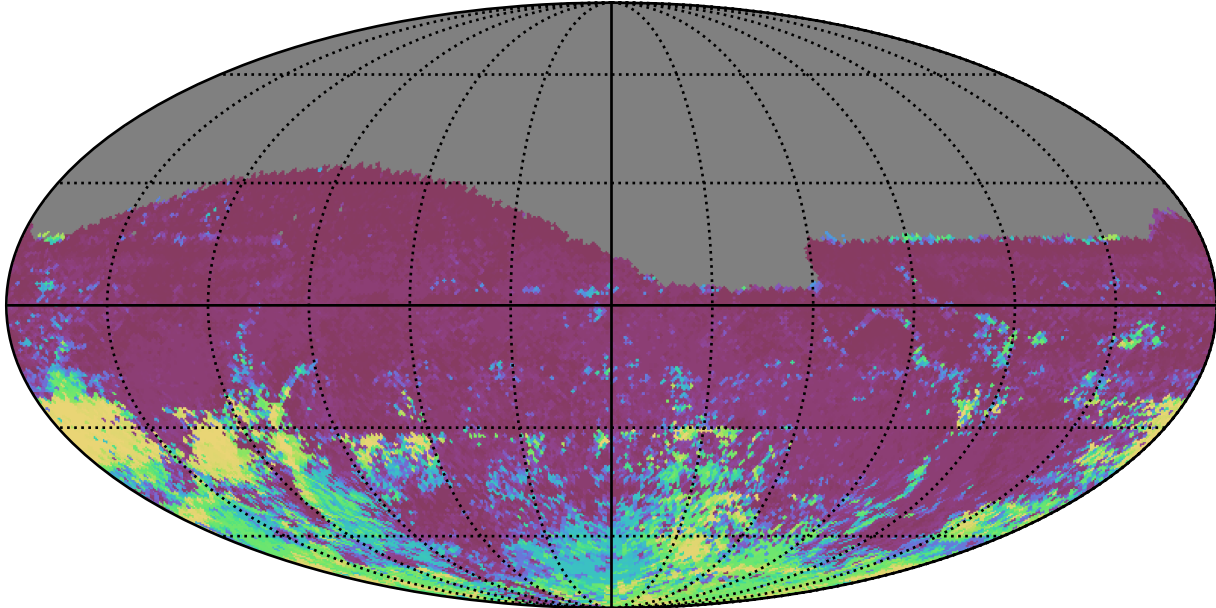
too_ignore_10_1v3.4_10yrs All sky r band: 75th Percentile Intranight Timespan
