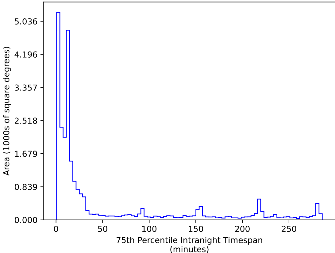
too_ignore_10_1v3.4_10yrs All sky r band: 75th Percentile Intranight Timespan
