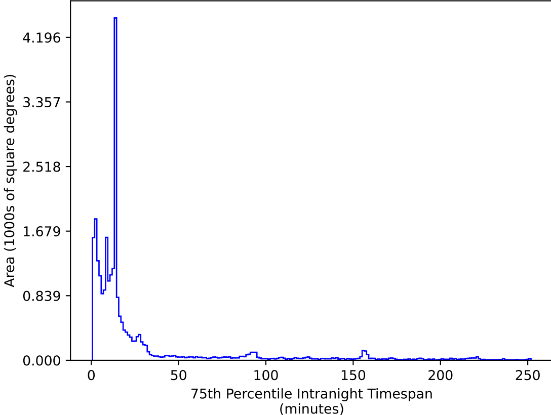
too_ignore_10_1v3.4_10yrs All sky i band: 75th Percentile Intranight Timespan
