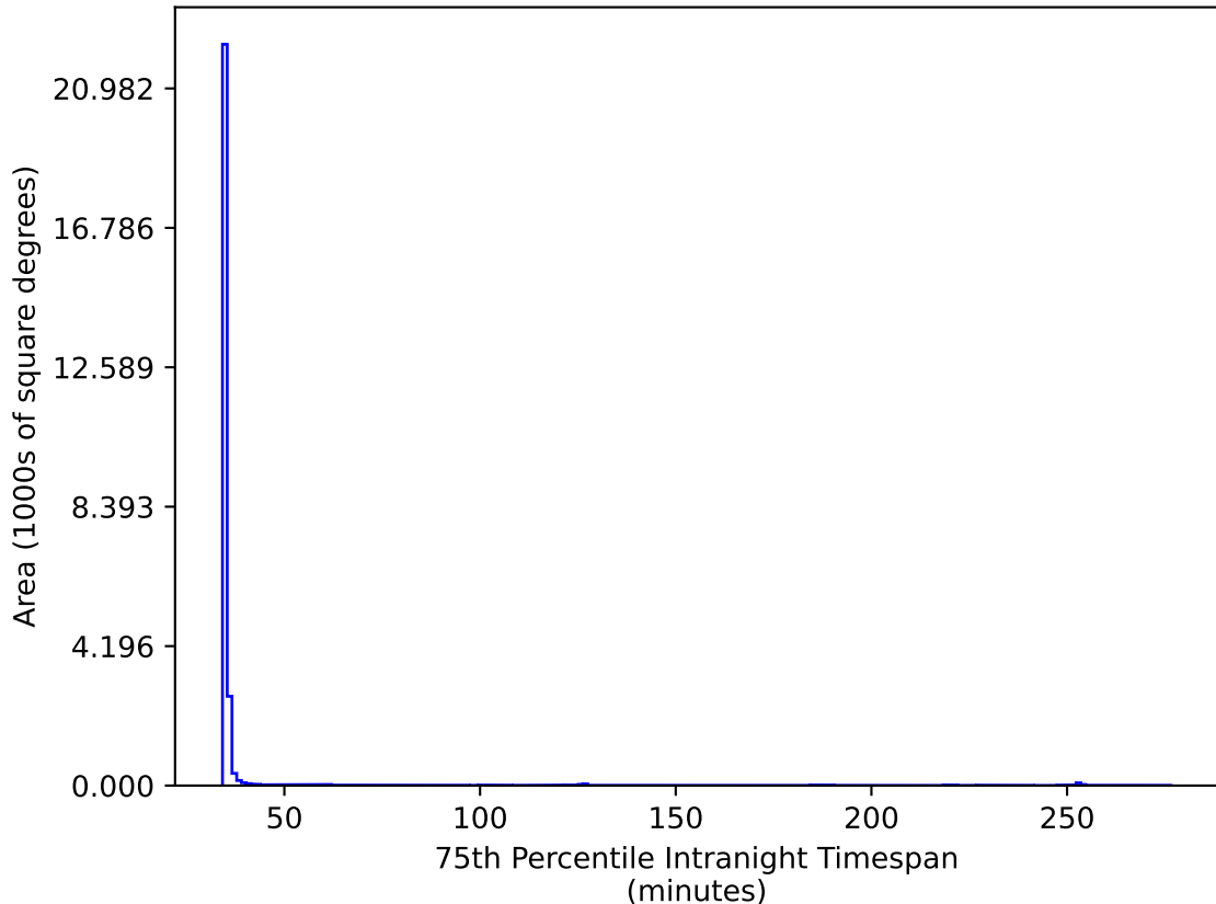
too_ignore_10_1v3.4_10yrs All sky gr bands: 75th Percentile Intranight Timespan
