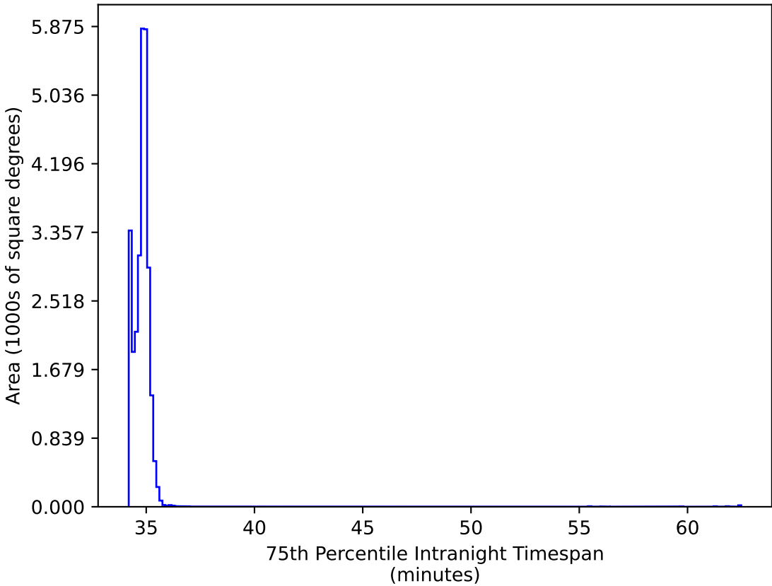
too_ignore_10_1v3.4_10yrs All sky: 75th Percentile Intranight Timespan
