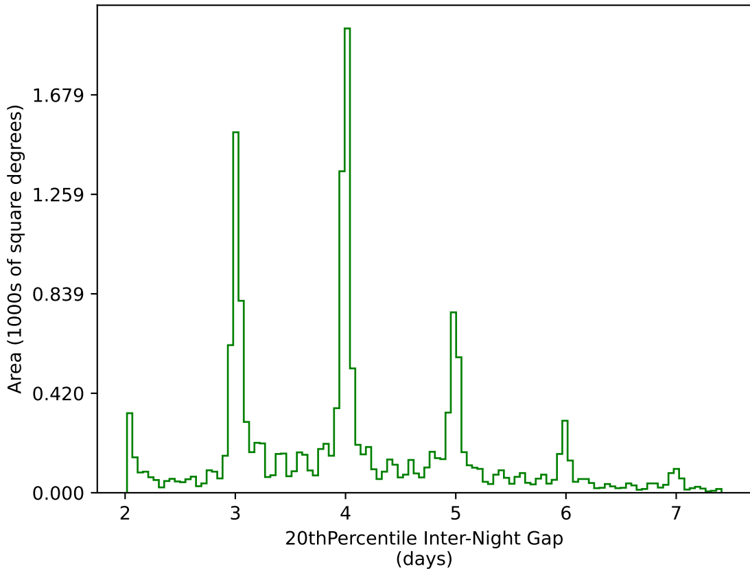
too_ignore_10_1v3.4_10yrs WFD g band: 20thPercentile Inter-Night Gap
